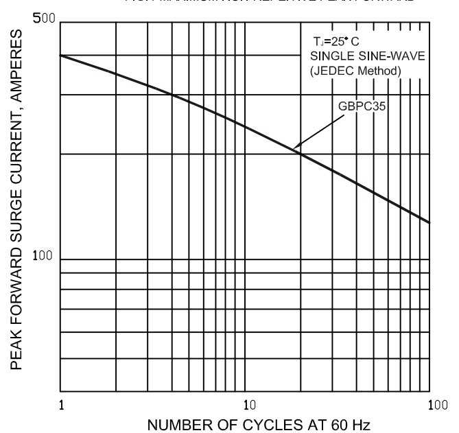
FIG.4-MAXIMUM NON-REPEITIVE PEAK FORWARD
